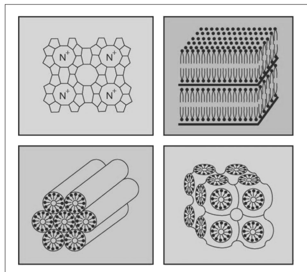
Figure 3: Structure of zeolite
